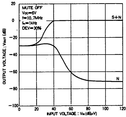
Fig. 16 FM detector output voltage (muting off) vs. input voltage
