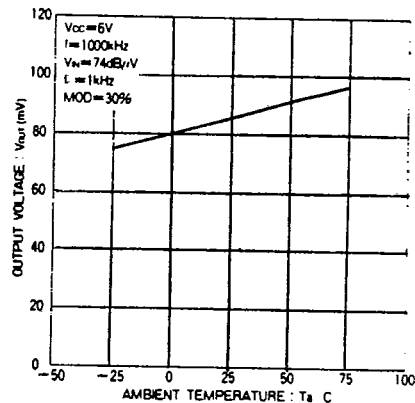
Fig. 27 AM detector output voltage vs. ambient temperature
