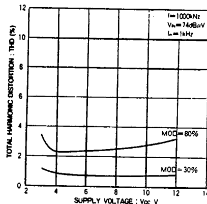
Fig. 30 AM total harmonic distortion vs. supply voltage
